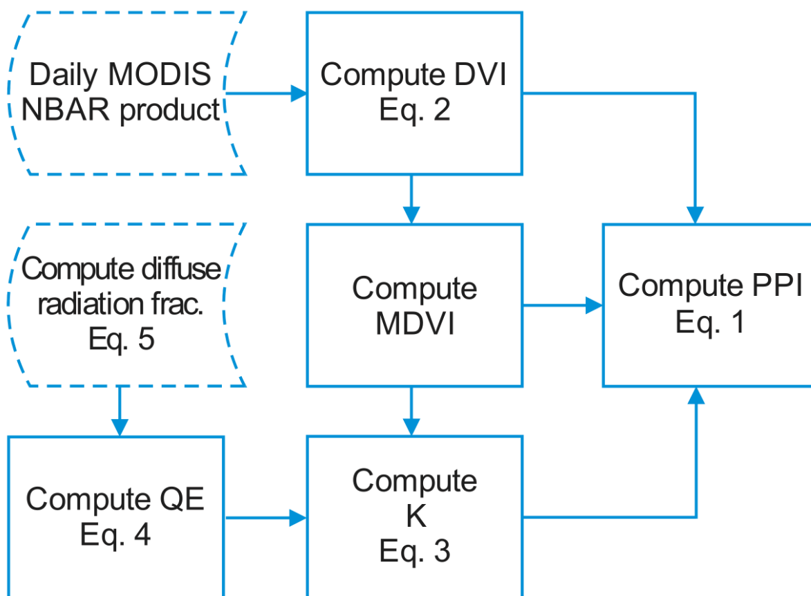
Figure 2. Processing flowchart for Plant Phenology Index (PPI) calculation
