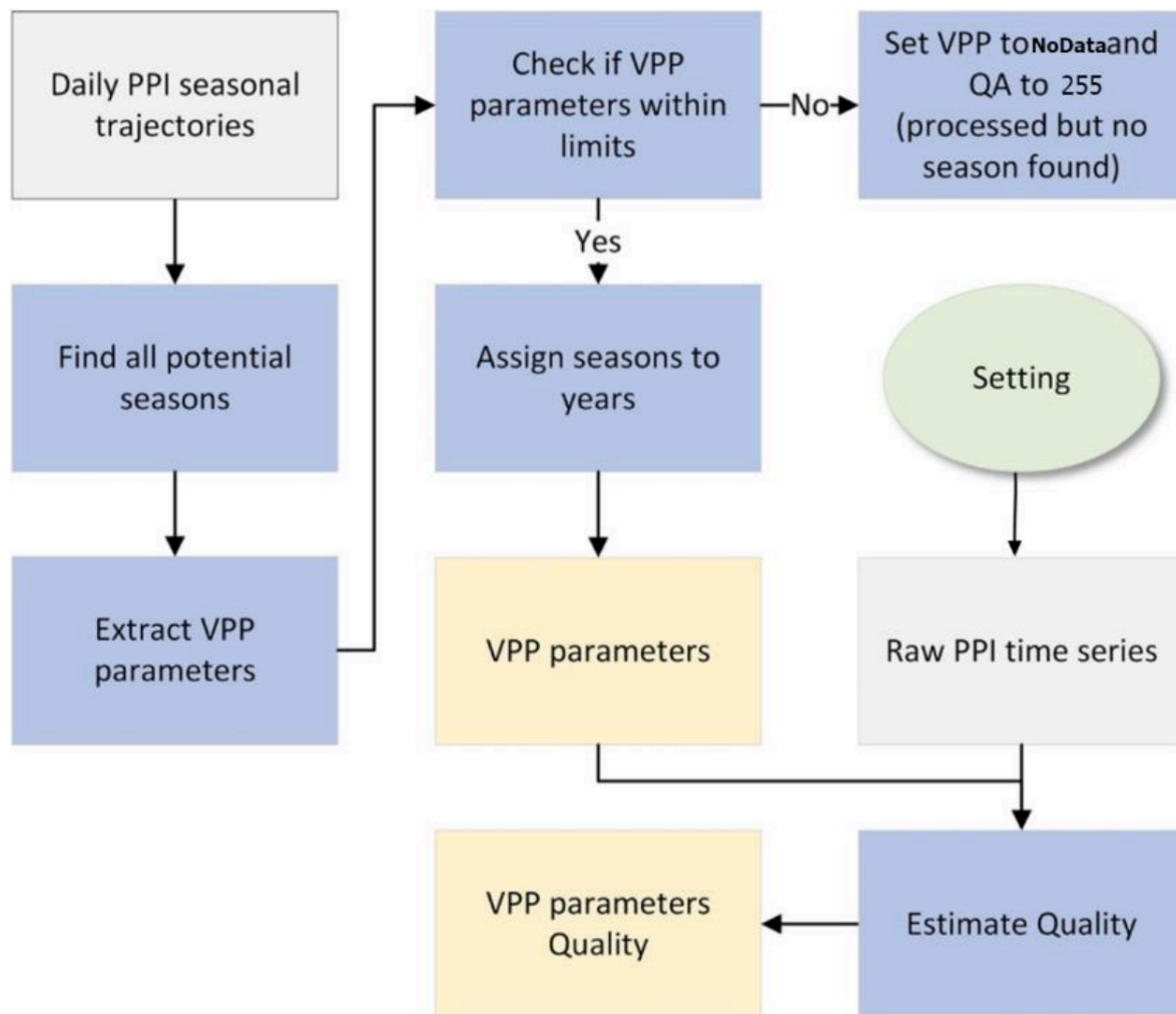
Figure 5. TIMESAT module for extracting phenological parameters.
