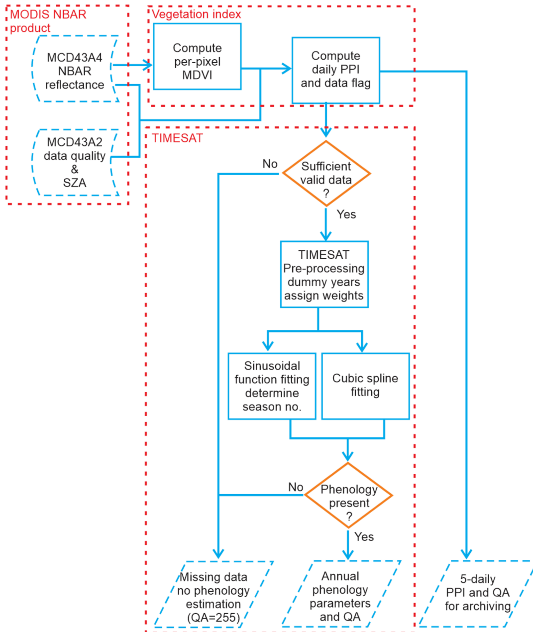
Figure 3. Processing overview of VPP and PPI time series, illustrated as a flowchart.
