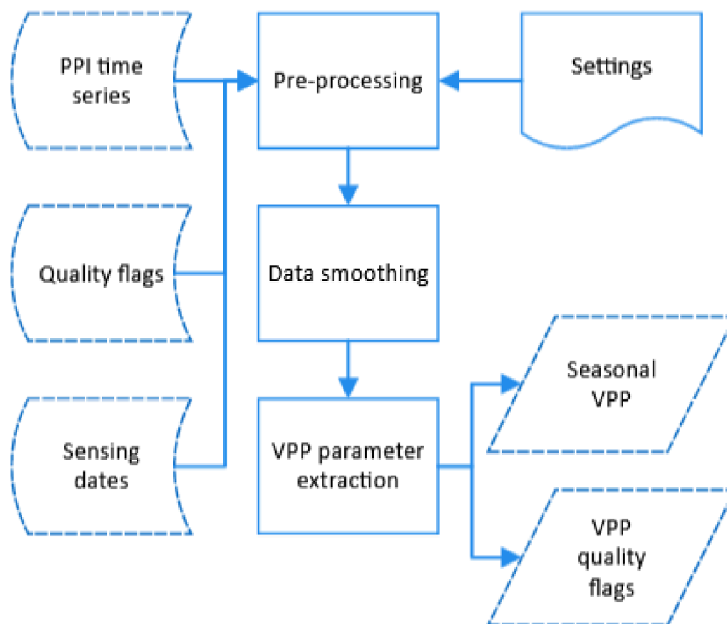
Figure 4. TIMESAT processing overview illustrated as a flowchart.
