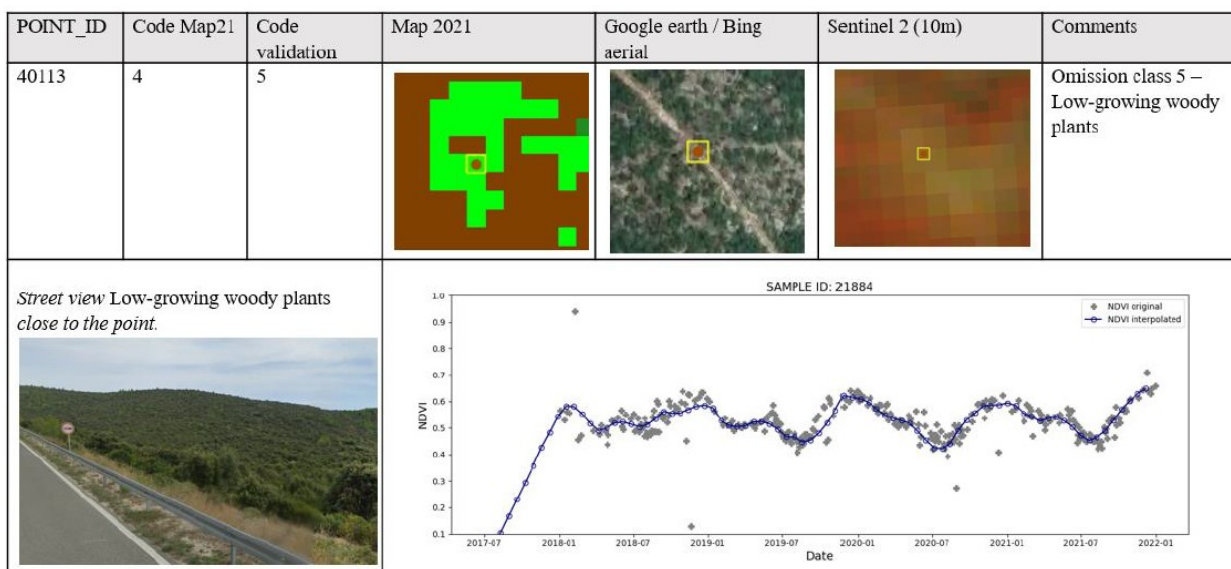
Figure 28: Example for class 4 commission in shrubby area
