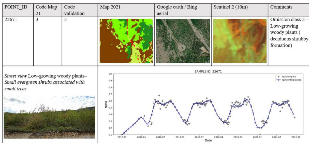
Figure 29: Example for class 3 commission in an area with deciduous shrubs
