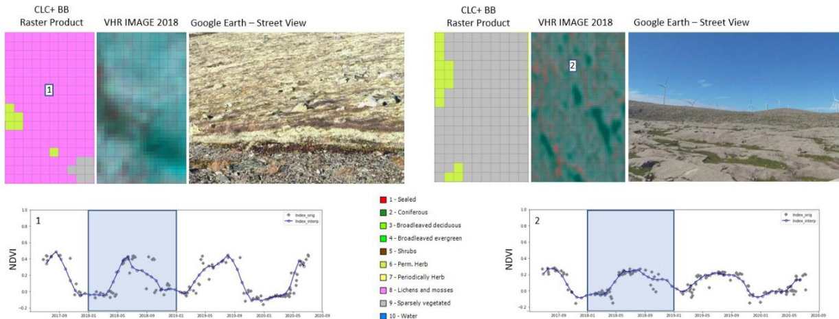
Figure 15: Example of the uncertainty in the mapping of Lichens and Mosses in the CLC+ Backbone Raster Product. These two examples from Southern Norway illustrate the typical similarity between surfaces covered by Lichens and Mosses versus Non- and Sparsely Vegetated areas with some fractions of sparse herbaceous vegetation. Both land cover compositions occur under similar biogeographic conditions and are nearly indistinguishable in VHR imagery or NDVI time-series.
