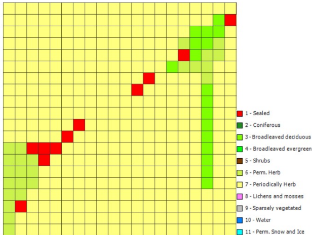
Figure 7: CLC+ BB Raster Product (left) and ESRI World Imagery (right) for a rural area in France illustrating the interruption of narrow linear elements which do not reach the majority per 10 m pixels (black grid lines) and typically show mixed spectral signals in the Sentinel-2 time series.
