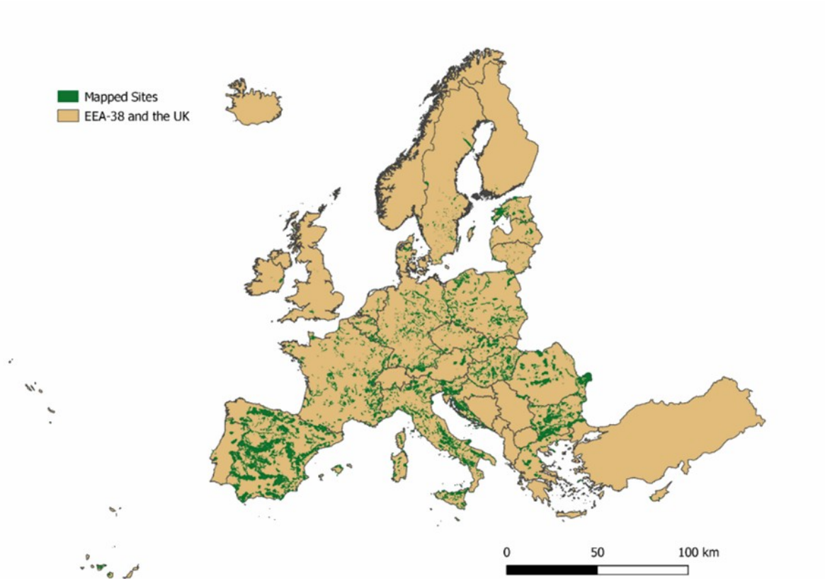
Figure 2: Coverage of the CLMS N2K product
